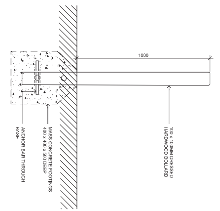
01 FIXED 100x100 HARDWOOD BOLLARD Scale 1:10
