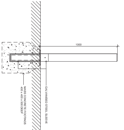
02 REMOVABLE 100x100 HARDWOOD BOLLARD Scale 1:10
