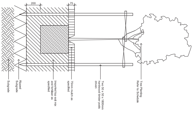
01 TREE PLANTING SCALE 1:10
